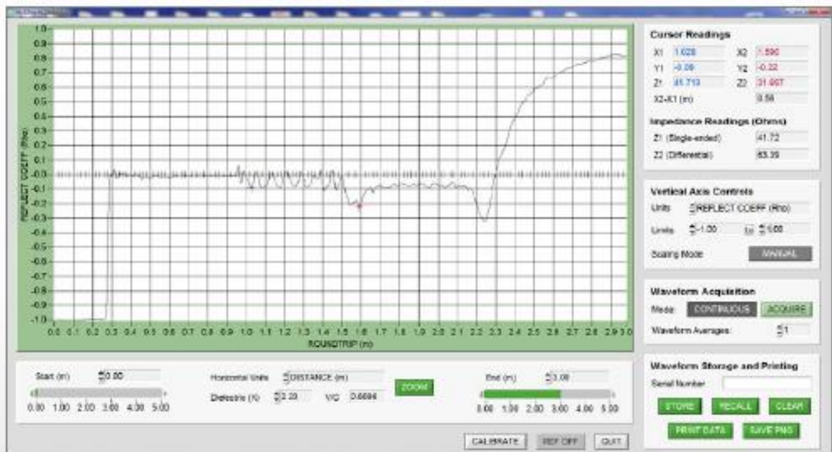
Example TDR reading of PC motherboard, accessed via USB port
